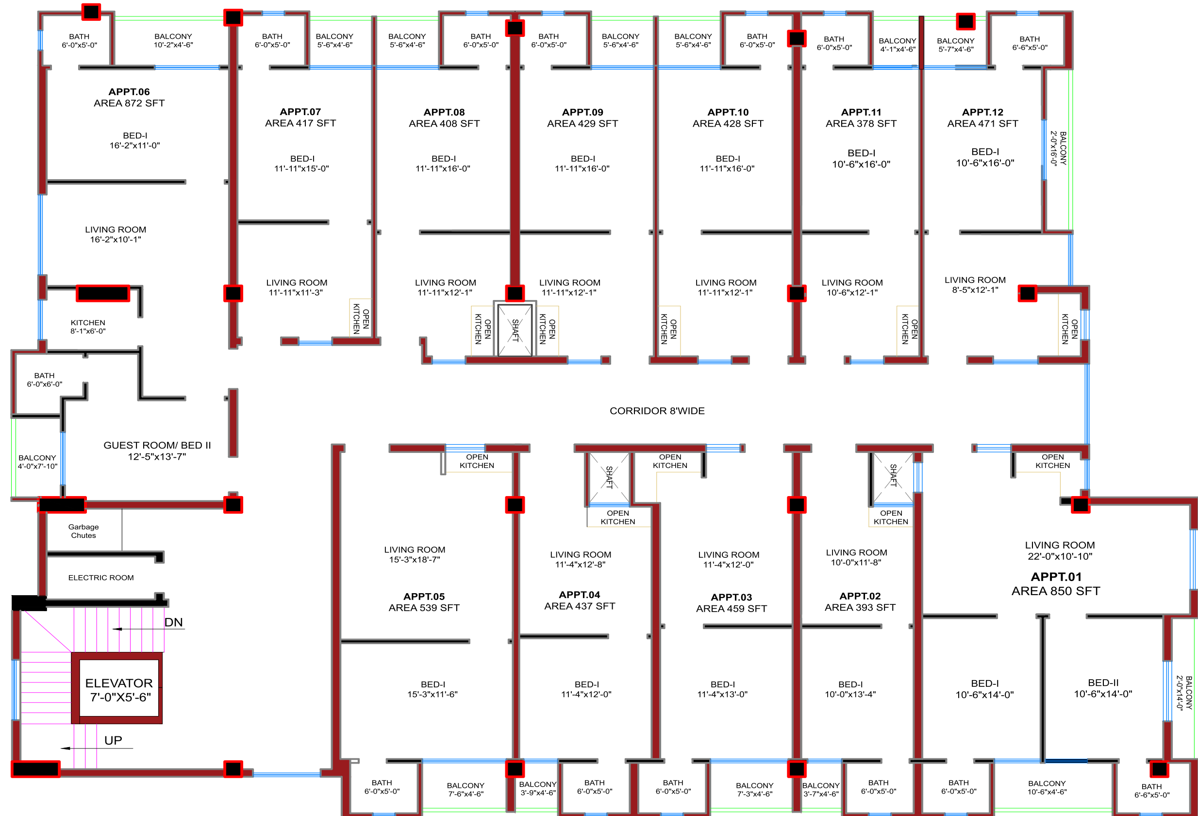
3rd Floor Plan
